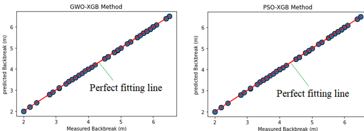
Figure 7. Comparison of correlation between predicted and actual values in the training dataset.
