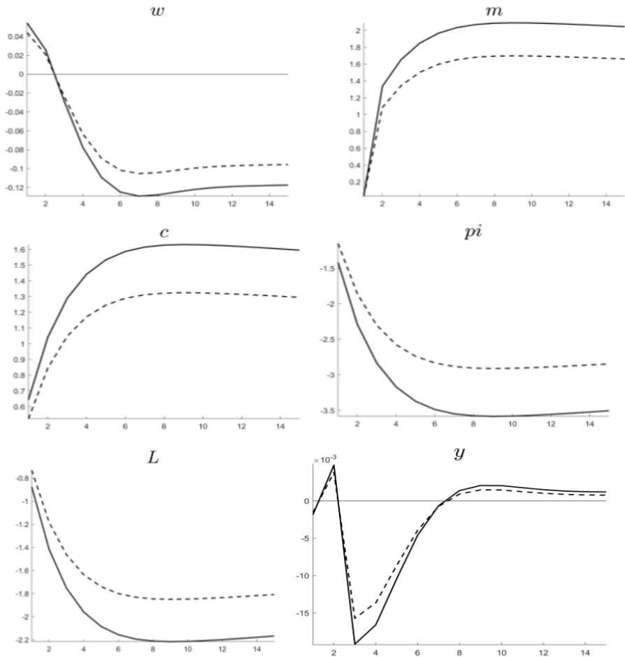
Figure 6. Impulse response from 1% shock to the interbank rate under 16.25% (Solid) and 20% (Dashed) liquidity ratio.
