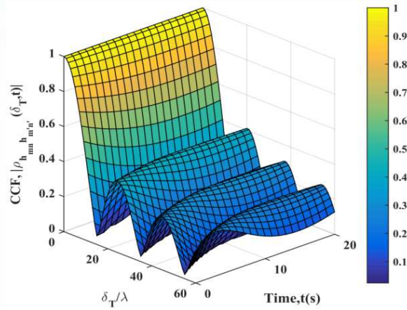
Fig. 12. Time-variant CCF of two distinct channels the antenna distance at BS.
