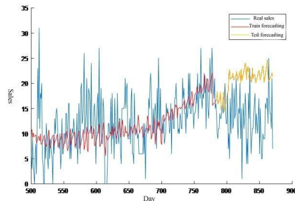
Fig. 6 The output related to the regression model as the initial forecast of minced meat product group
