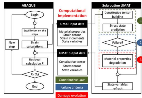
Fig. 2: The general algorithm of ABAQUS solver using UMAT [47]
