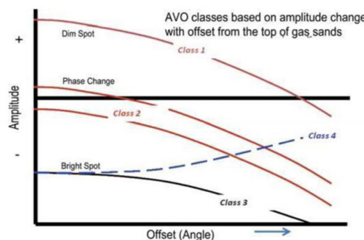
Fig. 1 Amplitude versus offset variation for four AVO classes [5].
