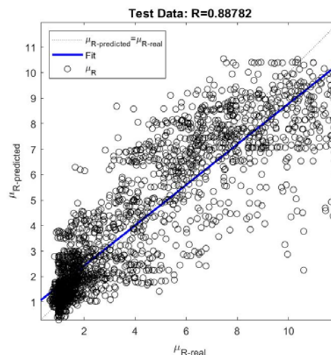
Fig. 5. Correlation between the real and predicted values (ANFIS model (2) - Subtractive clustering method) [17]
