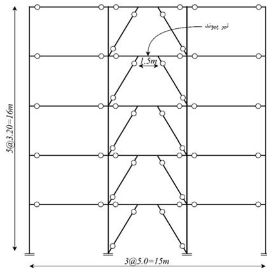
Fig. 7. 5-story steel frame example
