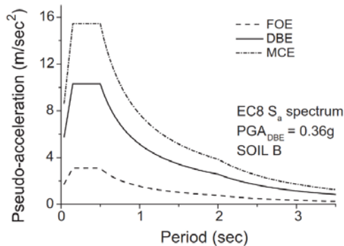
Fig. 8. Eurocode 8 elastic design spectrum [18]
