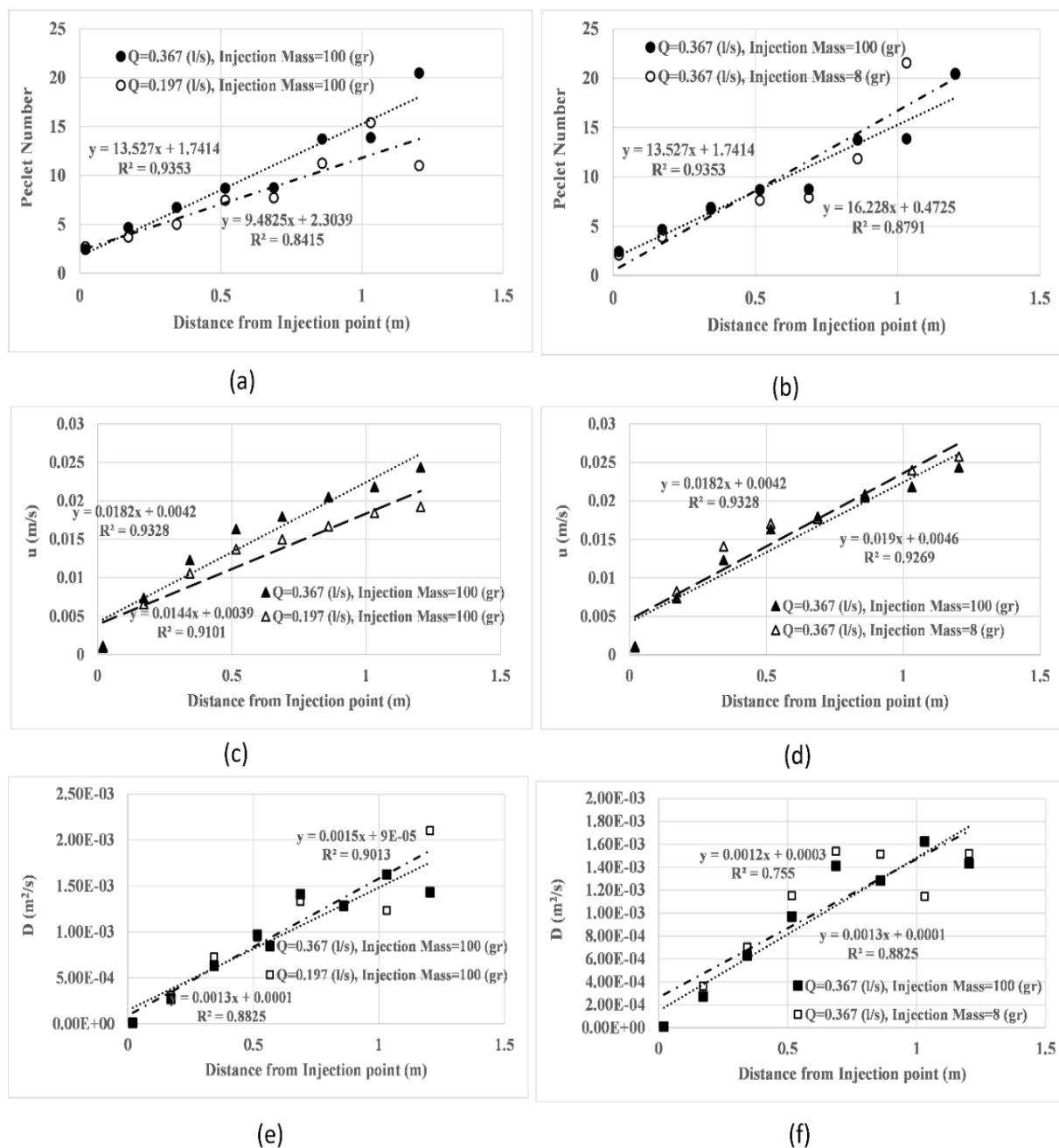
Fig. 8. a) Peclet number for different entrance discharges versus distance parameter, b) Peclet number for different entrance concentrations versus distance parameter, c) real crossing velocity for different entrance discharges versus distance parameter, d) real crossing velocity for different entrance concentrations versus distance parameter, e) dispersion coefficients for different entrance discharges versus distance parameter, f) dispersion coefficients for different entrance concentrations versus distance parameter
