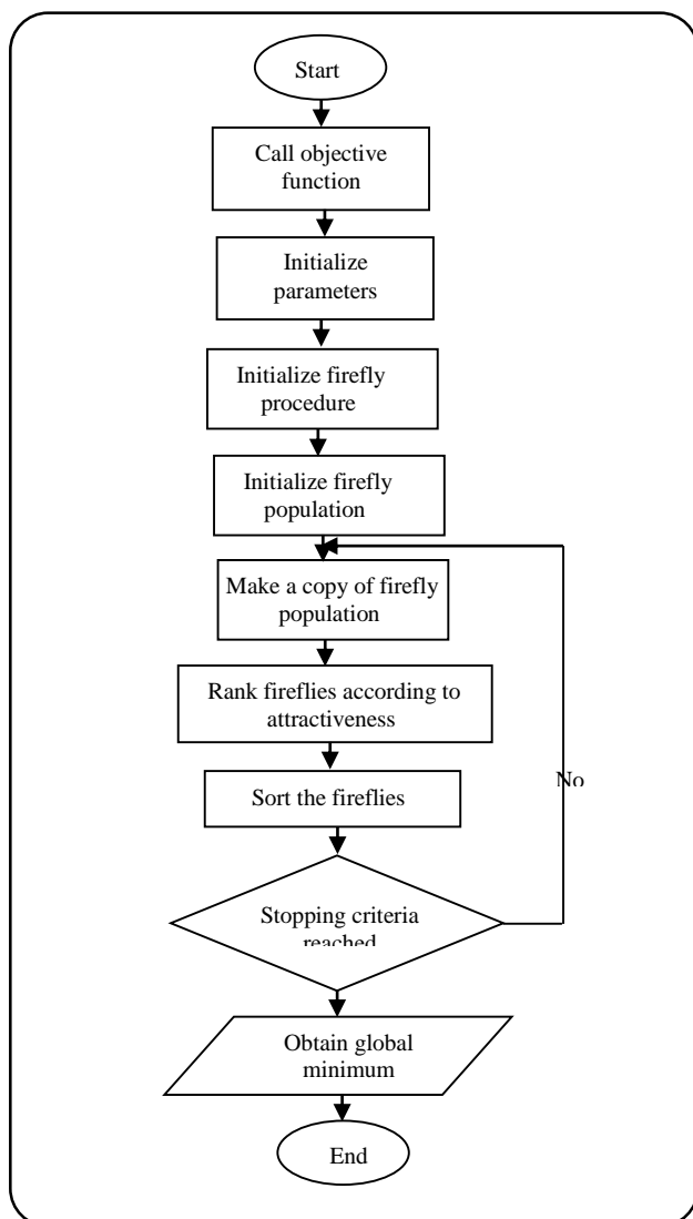
Fig. 3: Flowchart of FA algorithm.
