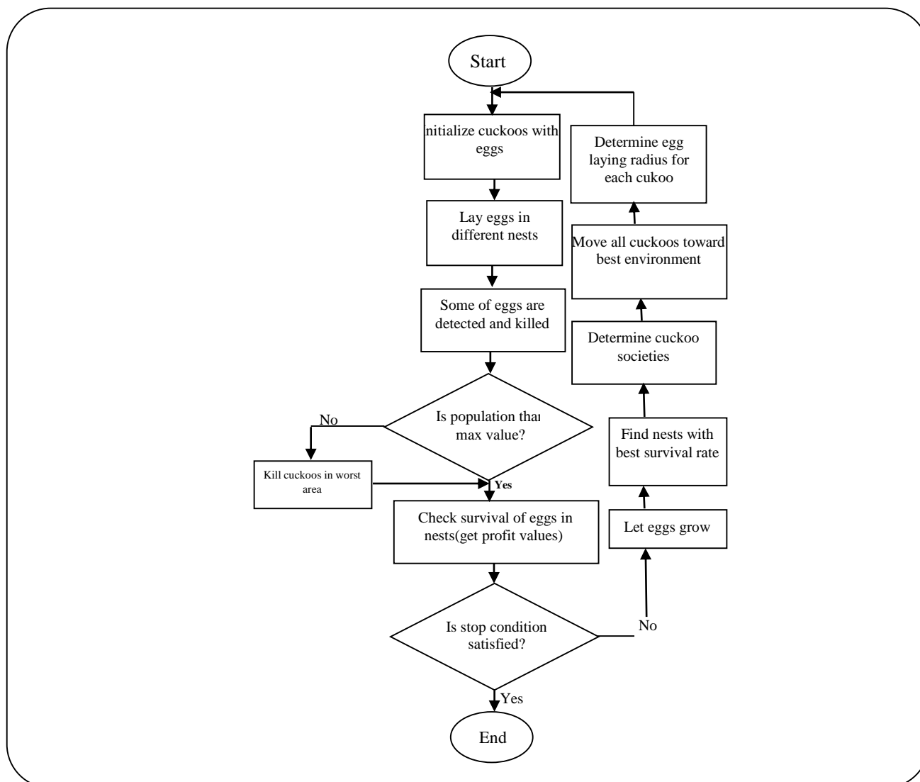
Fig. 2: Flowchart of Cuckoo Search algorithm.
