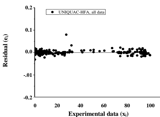
Fig. 12: Residual plots of tie-line of selected ternary systems.
