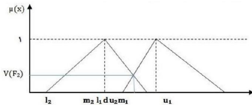
Figure 2: Fuzzy Model
