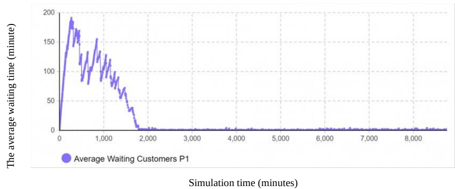
Figure 13. The average waiting time of customers to receive the radiator product in the current situation model with sustainability dimensions
