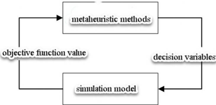
Figure 2. Simulation-optimization approach
