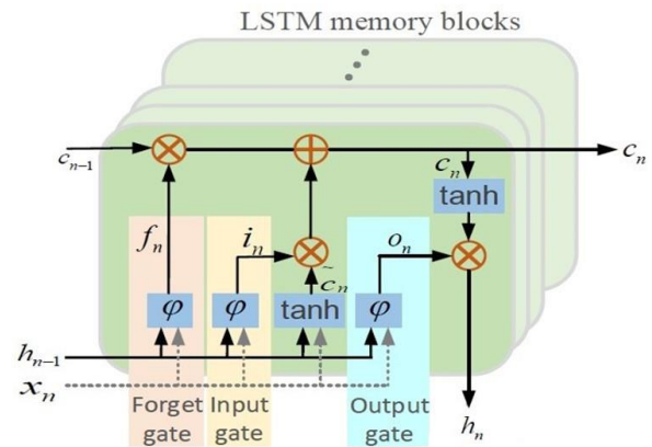
Figure 3: The overall structure of a LSTM model.
