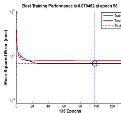
Bayesian Regularization
